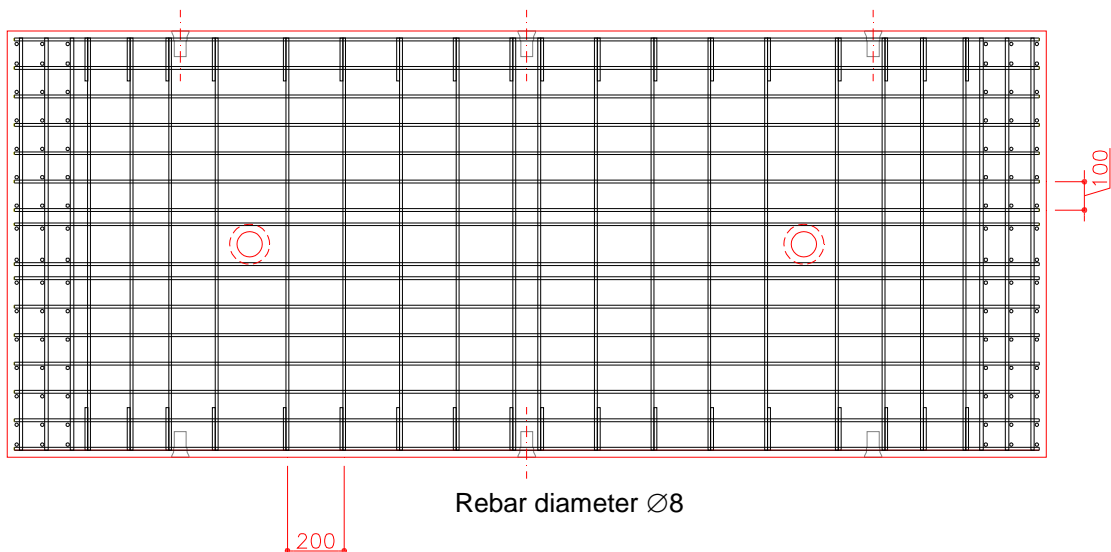
Fig. 2 – Tunnel segment reinforcement
