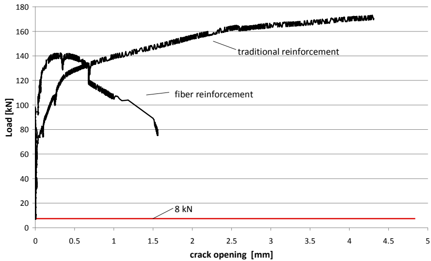
Fig. 8 – Flexural test: Load-crack opening
