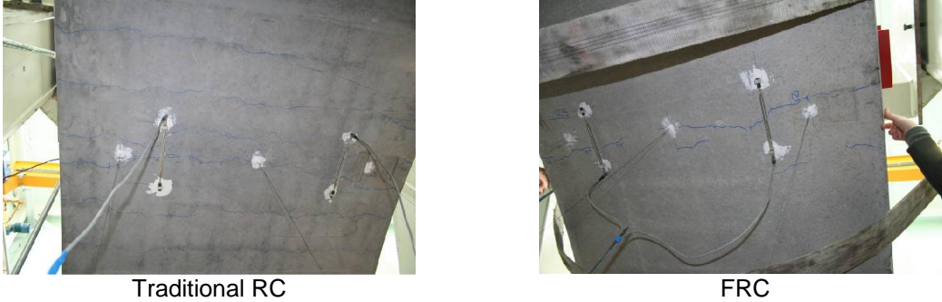
Fig. 9 – Crack patterns close to the failure
