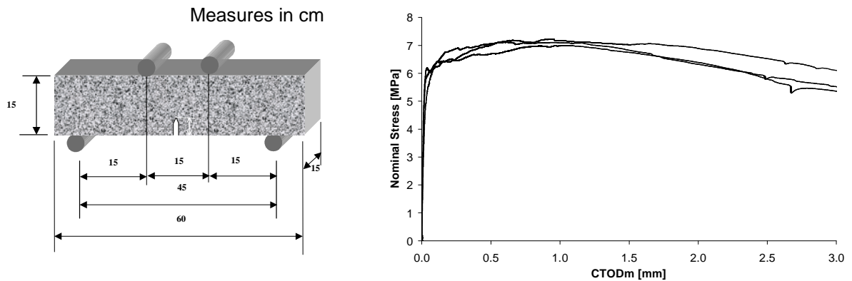
Fig. 3 - FRC behaviour in tension: a) test scheme; b) results: nominal strength-crack opening
