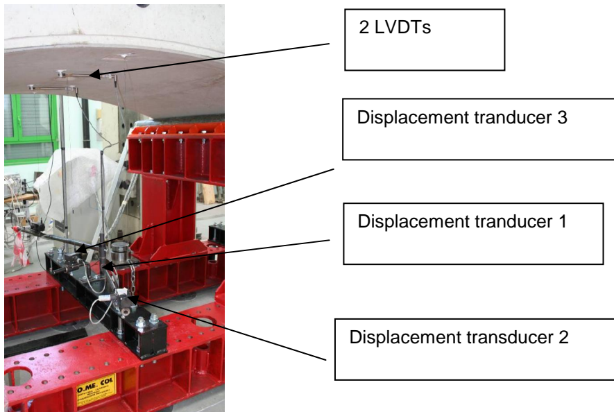
Fig. 5 – Measure instrumentation
