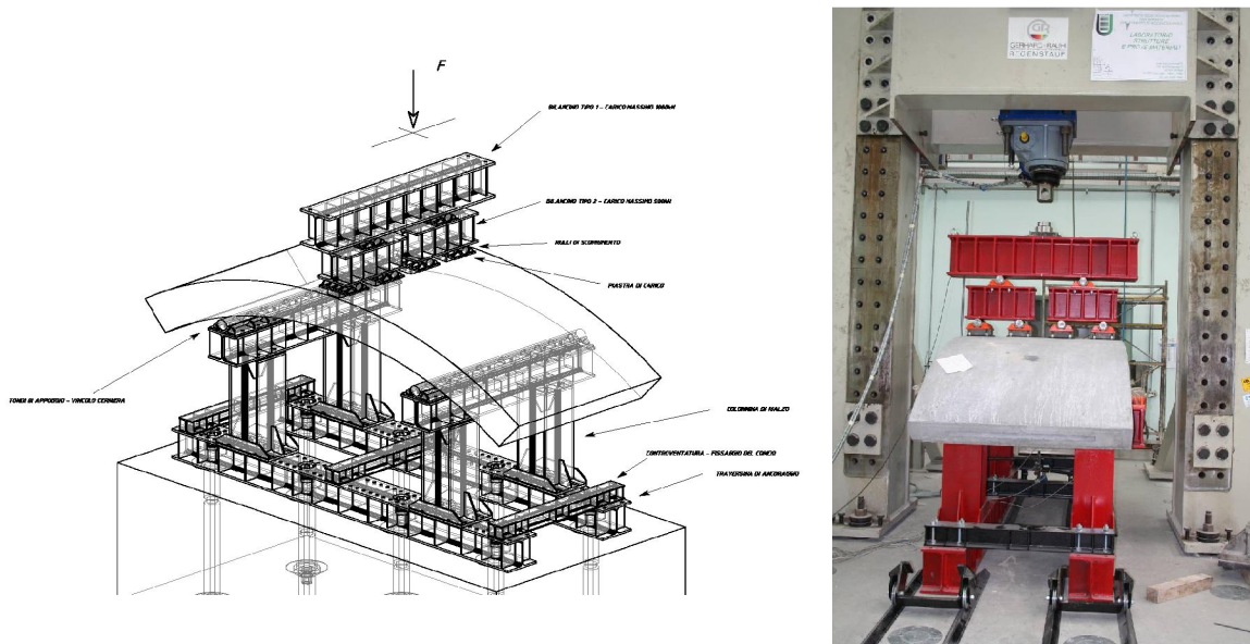
Fig. 4 – Flexural test set-up
