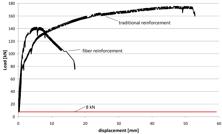
Fig. 7 – Flexural test: Load – midspan displacement
