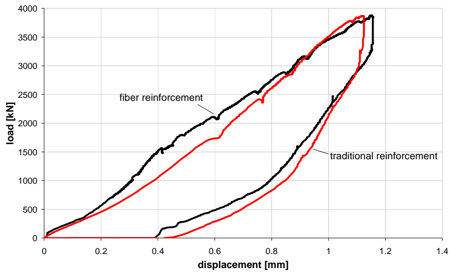
Fig. 10 – Results of the point load test
