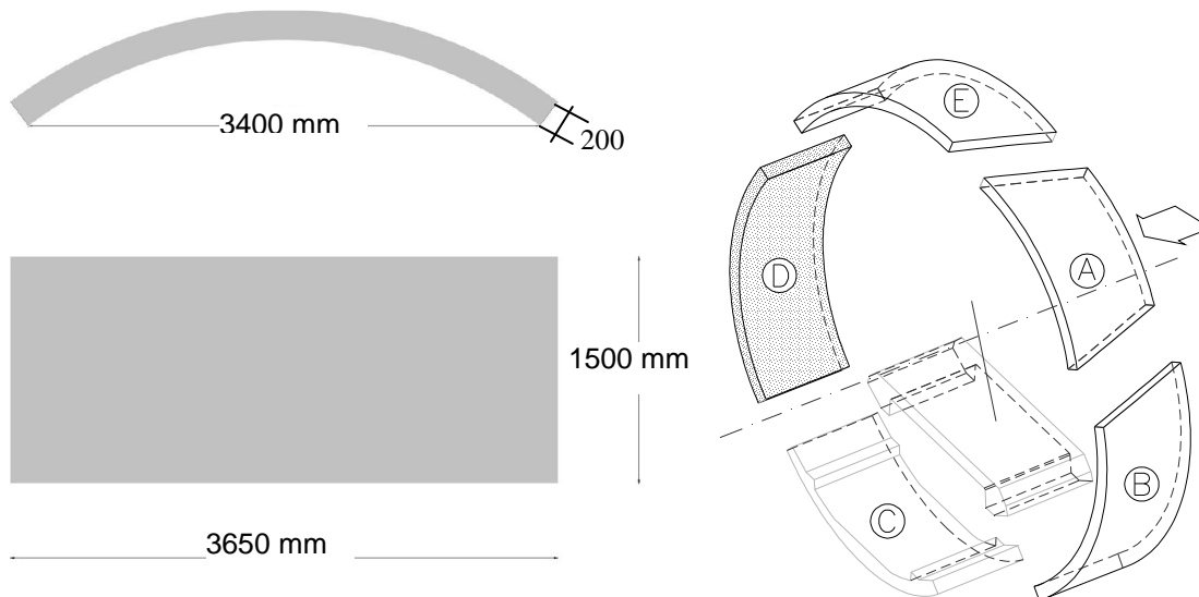
Fig. 1 - Tunnel segment geometry
