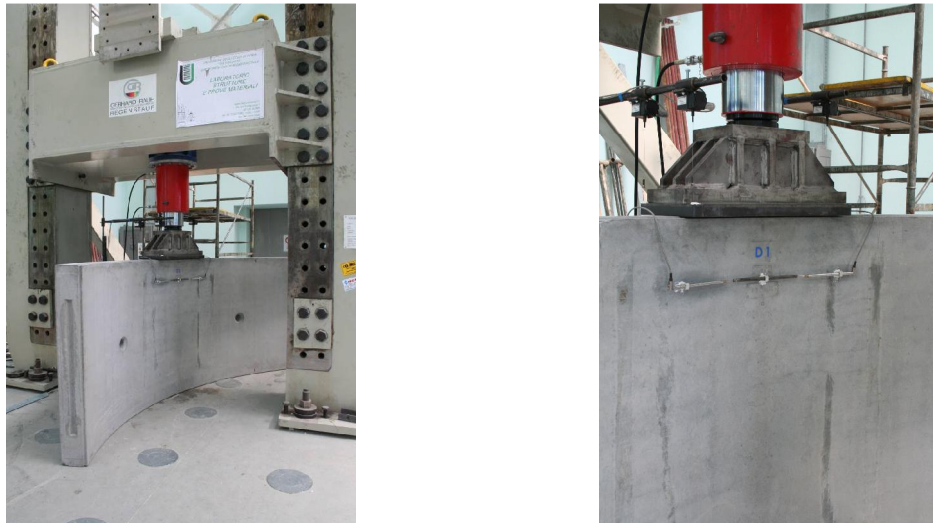
Fig. 6 – Point load test set up
